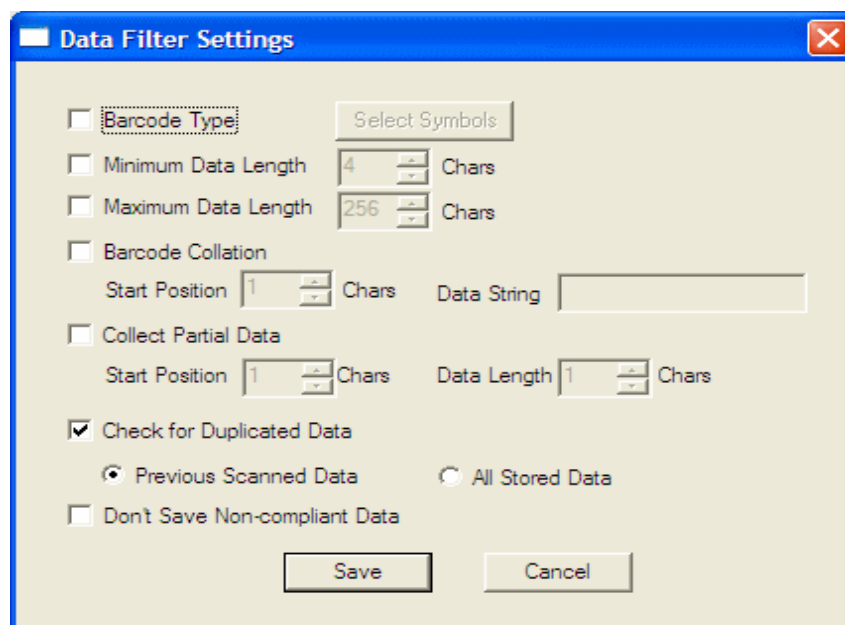
図 38-Data Filter Settings
