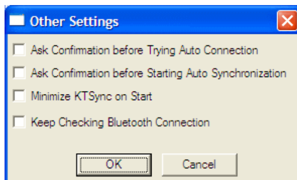
図 29-KTSync® Confirmation Settings
